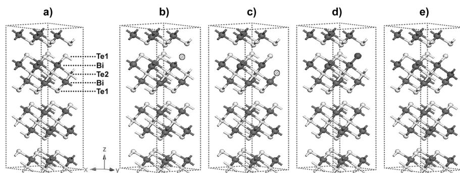
Figure 3. The model configurations of the \text{Bi}_2\text{Te}_3 supercell, with and without defects. a) Perfect hexagonal 2 \times 2 \times 1 \text{Bi}_2\text{Te}_3 supercell with quintuple layers with a sequence of Te1-Bi-Te2-Bi-Te1 along the c axis. b) A Te1 vacancy created by removing one Te1 atom, denoted as V_{\text{Te1}} . c) A Te2 vacancy from the removal of one Te2 atom, denoted as V_{\text{Te2}} . d) A Te1 antisite defect (one Te1 atom replaced by one Bi atom), denoted as \text{Bi}_{\text{Te1}} . e) A Te2 antisite defect (one Te2 atom replaced by a Bi atom), denoted as \text{Bi}_{\text{Te2}} . The white and gray spheres represent Te and Bi atoms, respectively, whereas the striated sphere shows the site where the atom was removed to generate a Te vacancy.
